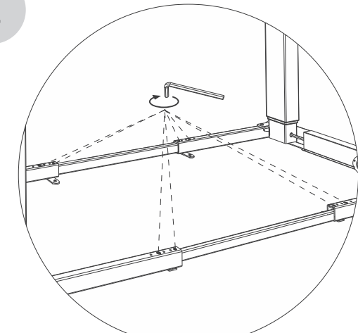
Pre-tighten screws
