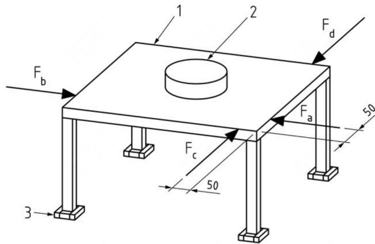
Fig. 28 Horizontal Durability Test
