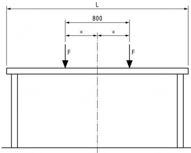
Fig. 11 Vertical Static Load Test for Tabletops over 1600 mm (63 in)
