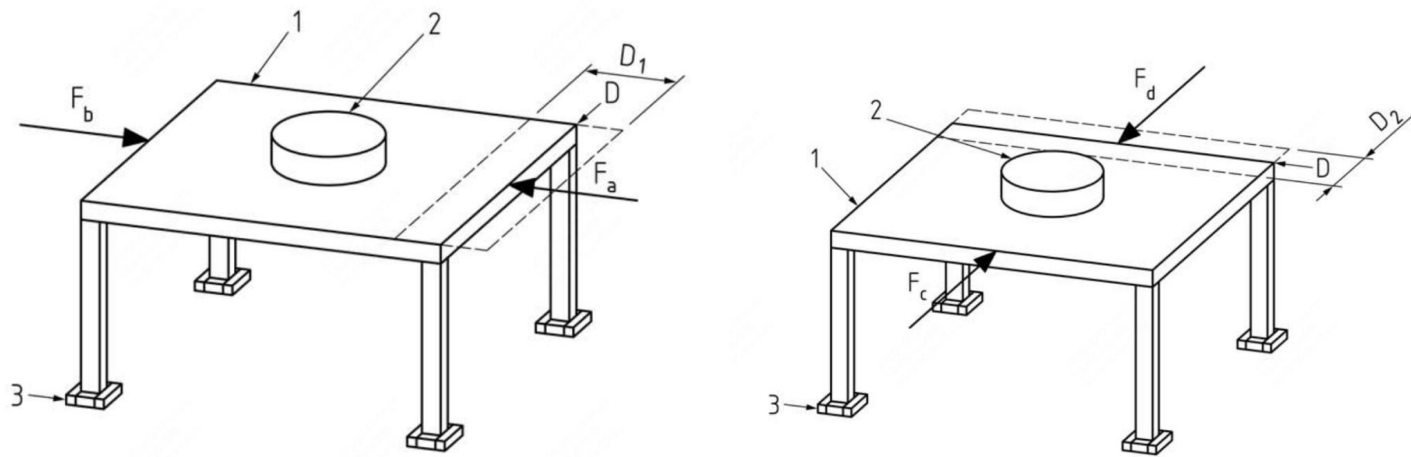
Fig. 7 Structural Rigidity Test
