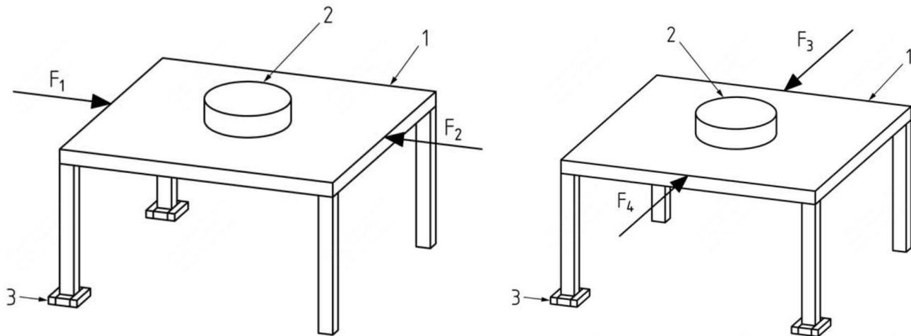
Fig. 8 Horizontal Static Load Test
