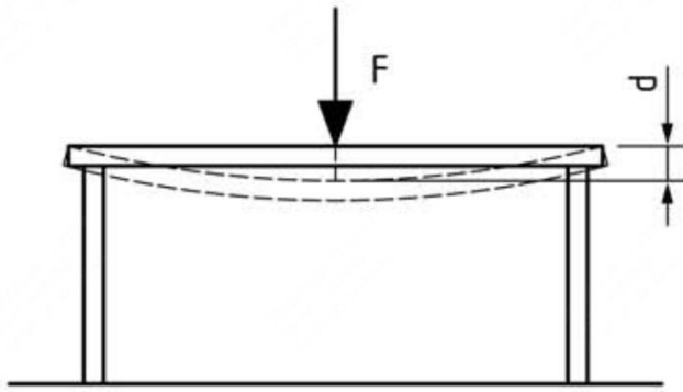
Fig. 9 Vertical Static Load Test
